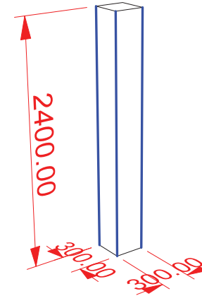
Corner Joint
